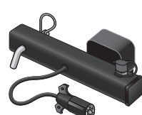
FS7015PC-BU 2 in. Hitch Mount with Threaded Hex Base, 24 in. Power Cord with 7-Way Plug and Backup Alarm
